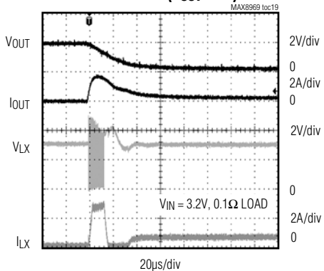
HARD-SHORT ( V_{OUT} = 5V )
