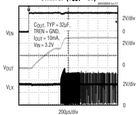
STARTUP ( V_{OUT} = 5V )
