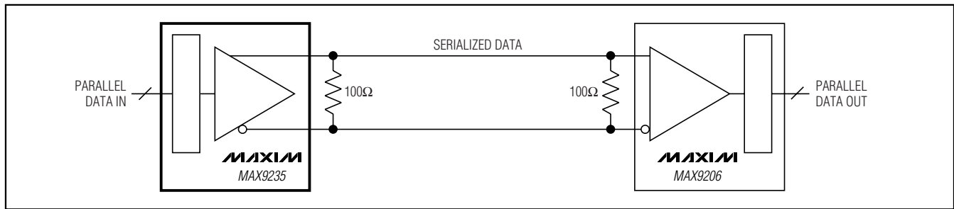
Figure 8. Double-Terminated Point-to-Point
