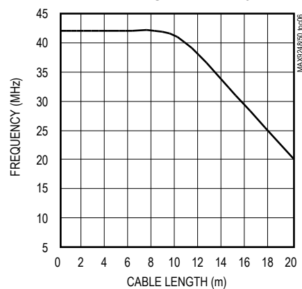
CABLE LENGTH vs. FREQUENCY BIT-ERROR RATE < 10^{-9}
