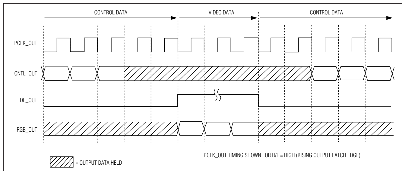
Figure 18. Output Timing
