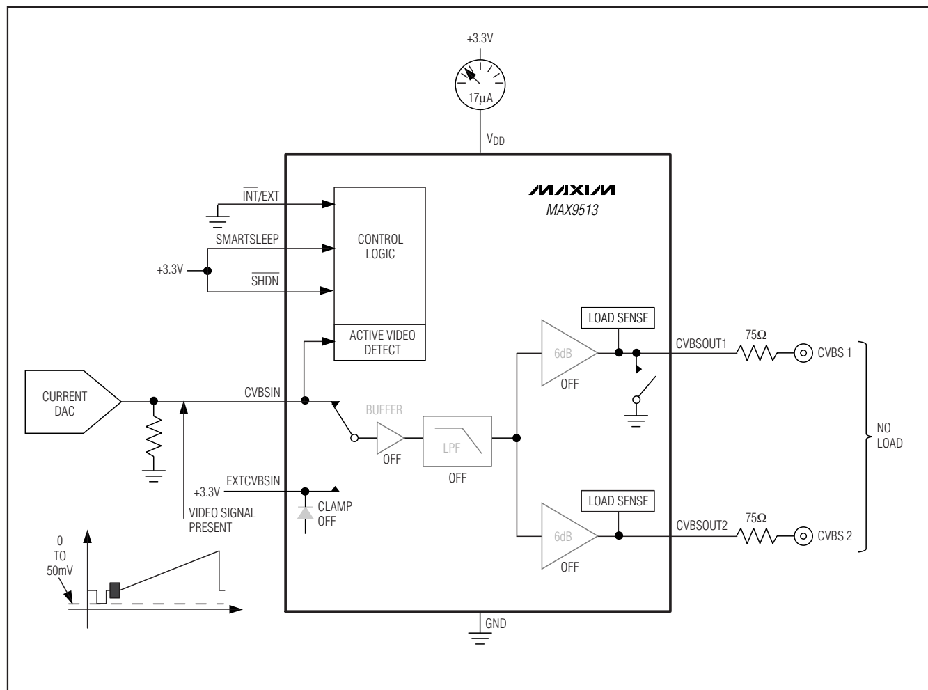
Figure 3. Active-Detect Mode with No Output Loads
