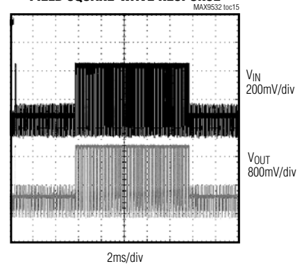
FIELD SQUARE-WAVE RESPONSE
