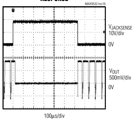
OUTPUT SHORT-TO-BATTERY RESPONSE
