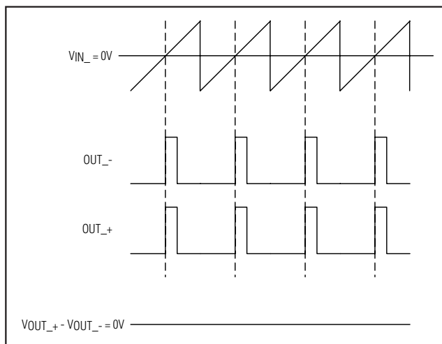
Figure 4. MAX9701 Outputs with No Input Signal
