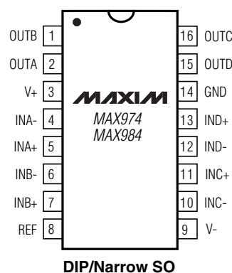
DIP/Narrow SO
