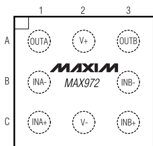
UCSP
