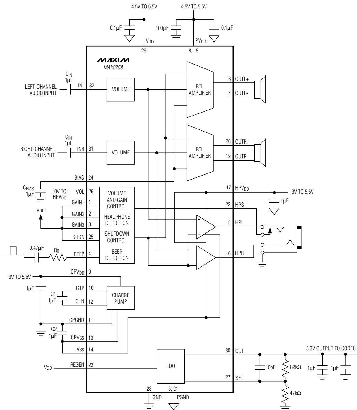
FIGURE SHOWN WITH SPKR GAIN = 25.5dB, LDO SHOWN IN ADJUSTABLE OUTPUT MODE SET TO 3.3V, HP GAIN = 3dB.
