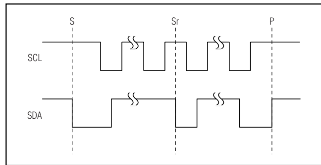
Figure 4. START/STOP Conditions
