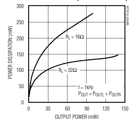
POWER DISSIPATION vs. OUTPUT POWER (HEADPHONE MODE)
