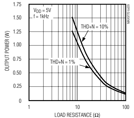
OUTPUT POWER vs. LOAD RESISTANCE (SPEAKER MODE)
