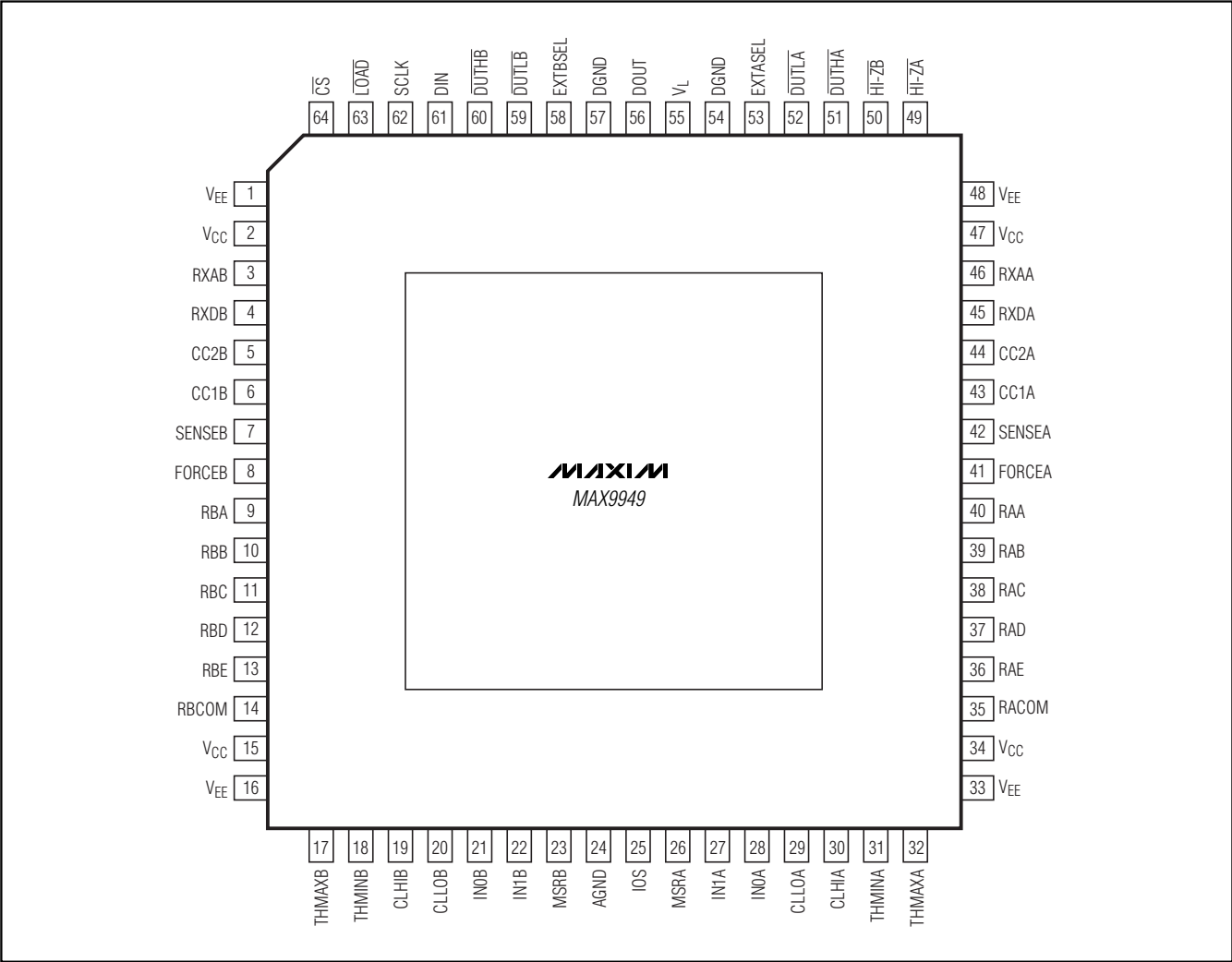
MAX9949 Pin Configuration
