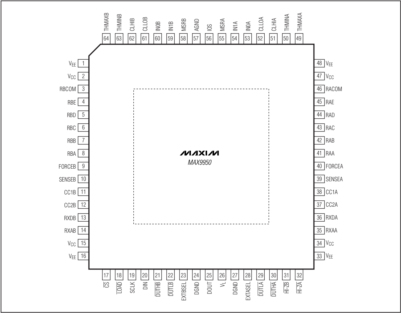
MAX9950 Pin Configuration
