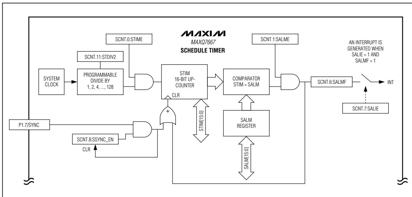
Figure 8. Schedule-Timer Module Block Diagram
