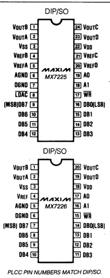
Pin Configurations
