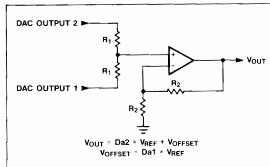
Figure 10. Offset Circuit
