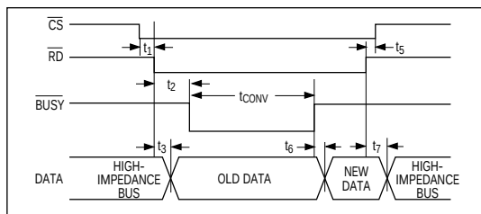
Figure 3. Slow-Memory Interface Timing Diagram
