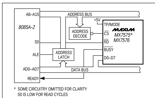
Figure 4. MX7575/MX7576 to 8085A-2 Slow-Memory Interface
