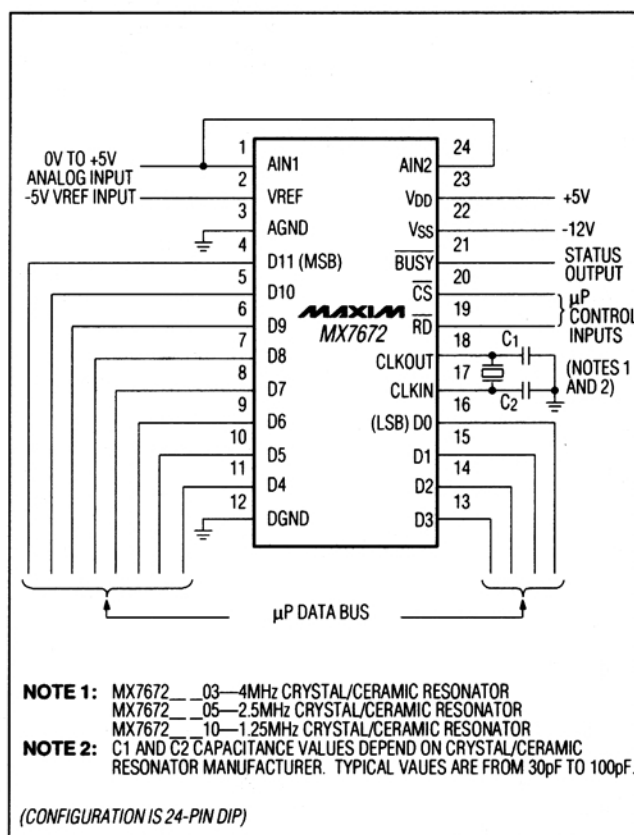
Figure 3. MX7672 Operational Diagram
