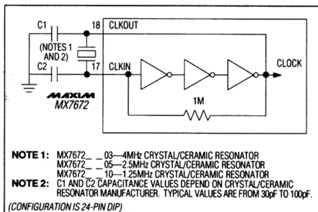
Figure 6. MX7672 Internal Clock Circuit
