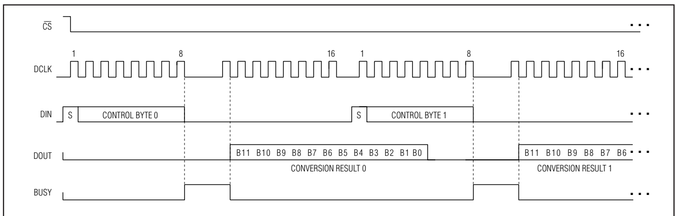
Figure 11. 16-Clock/Conversion Timing
