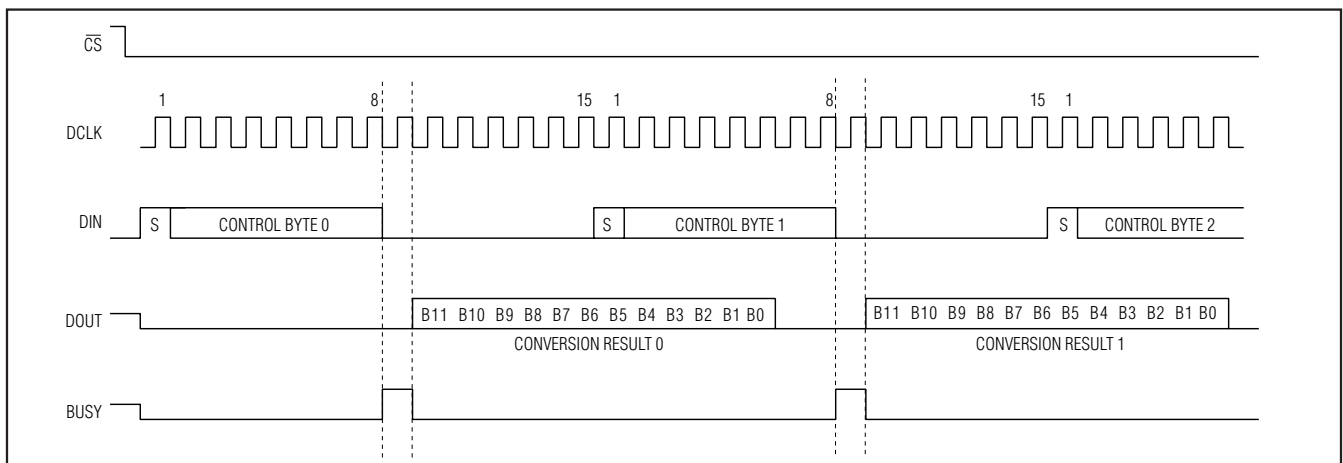
Figure 10. 15-Clock/Conversion Timing
