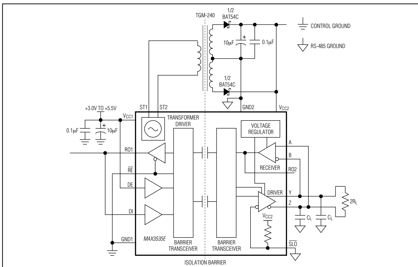
Figure 5. Self-Oscillating Configuration
