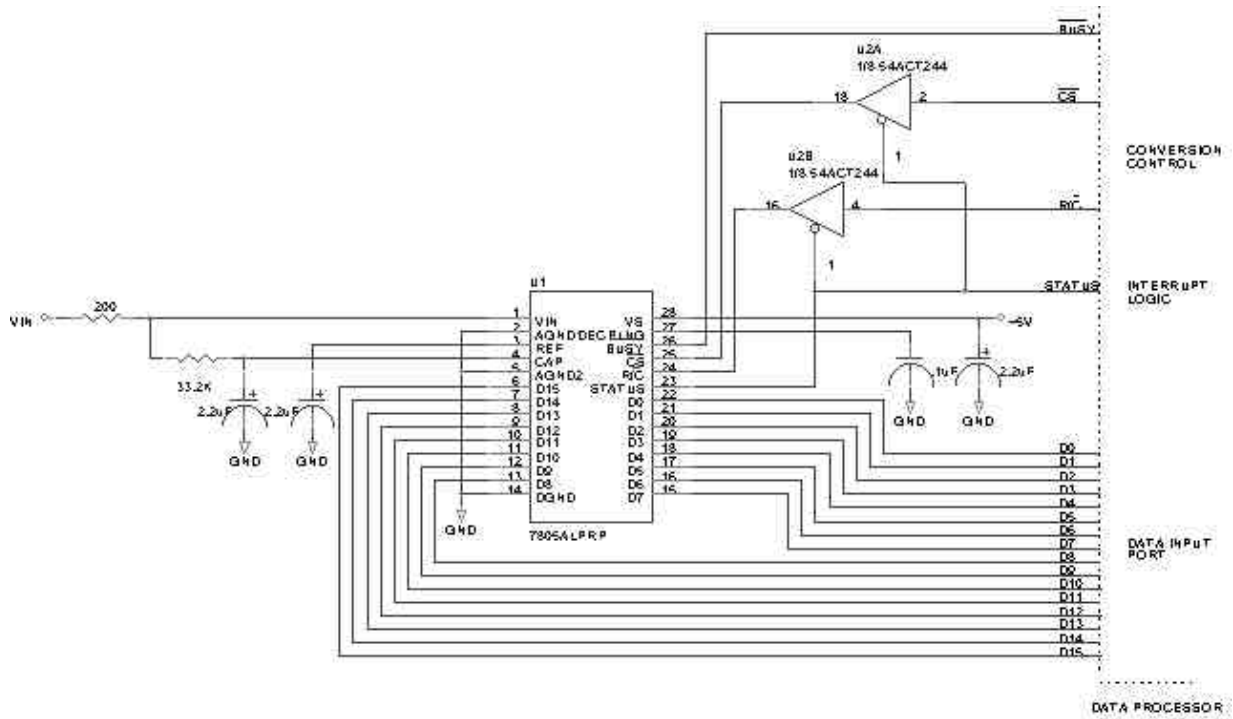
FIGURE 3. TYPICAL 7805ALPRP APPLICATION CIRCUIT
