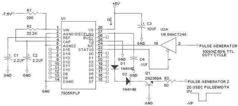
FIGURE 6. LPT™ TEST CIRCUIT
