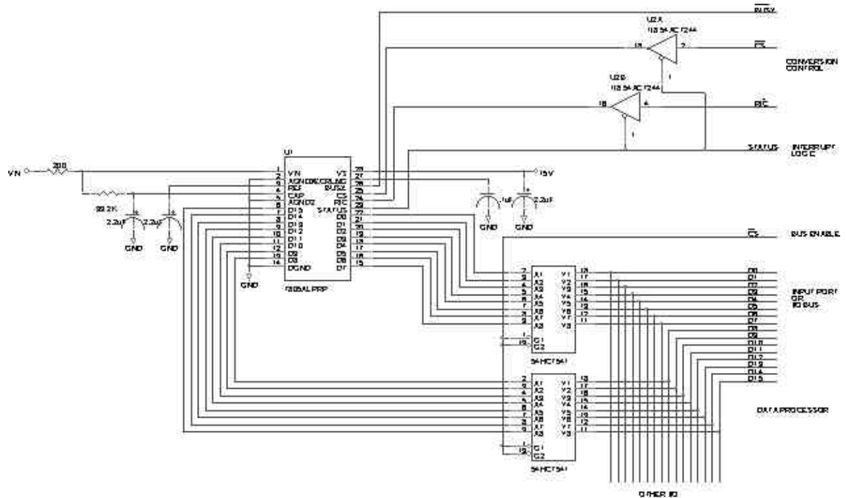
FIGURE 4. TYPICAL 7805ALPRP CIRCUIT WITH 16-BIT BUS INTERFACE
