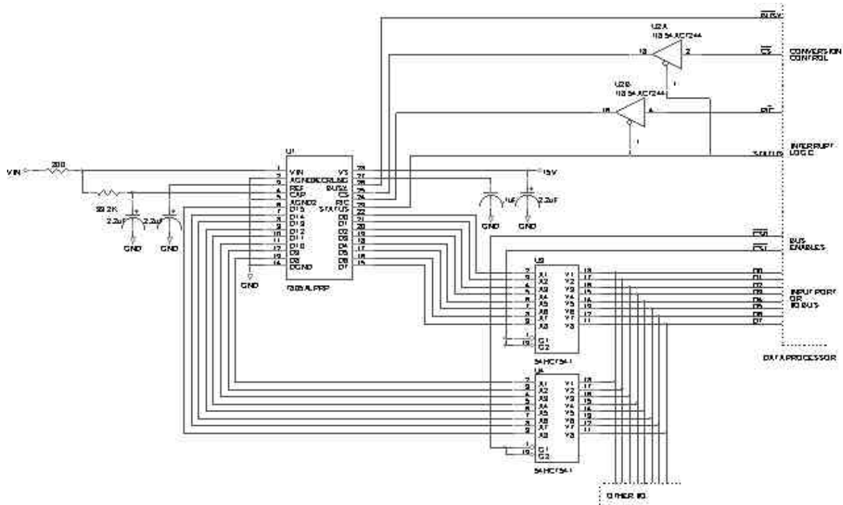
FIGURE 5. TYPICAL 7805ALPRP CIRCUIT WITH 8-BIT BUS INTERFACE
