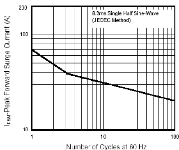
Fig.4 - Maximum Non-Repetitive Forward Surge Current Uni-Directional Only
