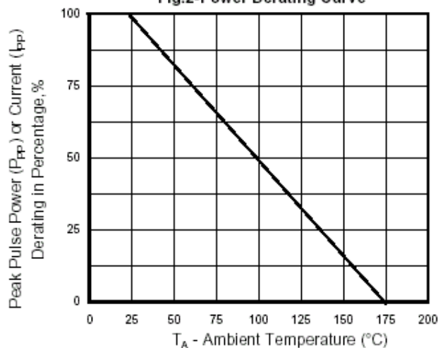
Fig.2-Power Derating Curve
