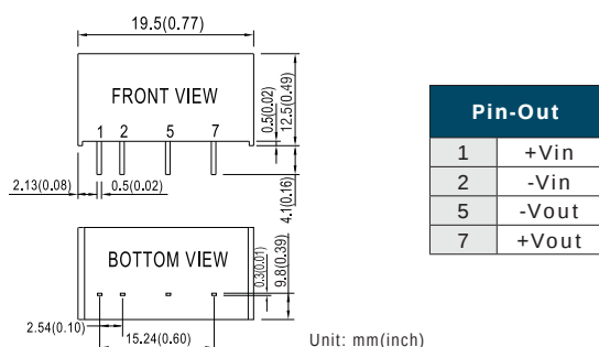
▲ MDS02 0.77" x 0.39" x 0.49"
