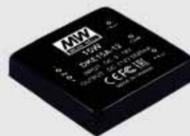
▲ DKE15 2" x 2" x 0.43"
