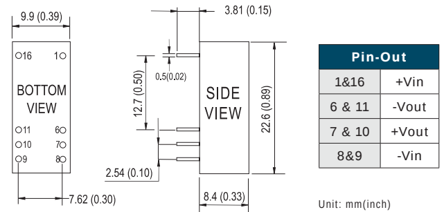
▲ SUS01 0.89" x 0.39" x 0.33"
