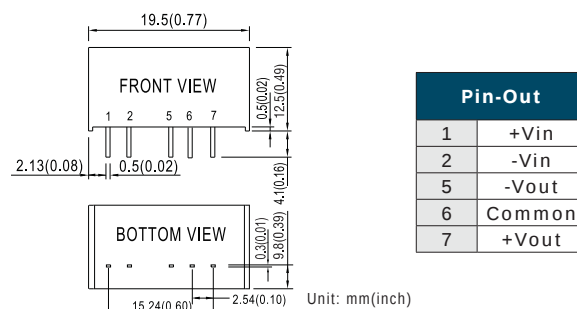
▲ MDD02 0.77" x 0.39" x 0.49"
