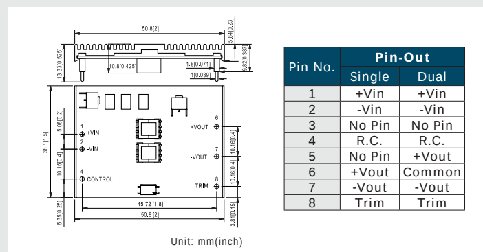
▲ NSD15-S 2" x 1.5" x 0.387"
