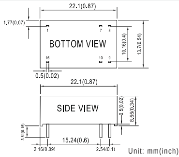
▲ SLC03 0.87" x 0.54" x 0.34"
