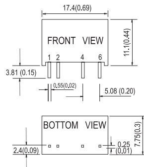
▲ SPA01 0.69" x 0.3" x 0.44"
