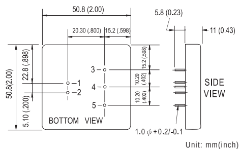
▲ SKE15 2" x 2" x 0.43"
