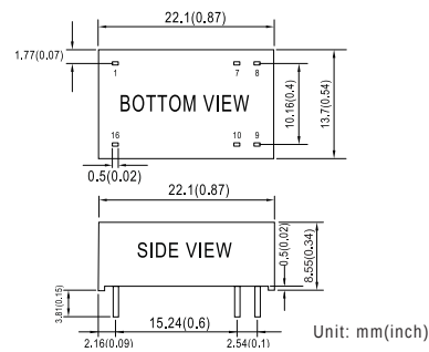
▲ DLC03 0.87" x 0.54" x 0.34"
