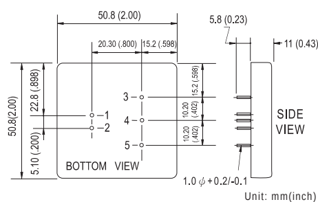
▲ DKE15 2" x 2" x 0.43"
