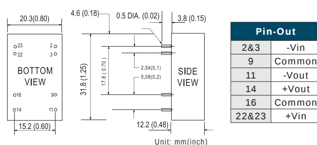
▲ DCW05 1.25" x 0.80" x 0.48"
