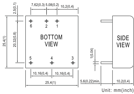
▲ SKMW20 1" x 1" x 0.40"
