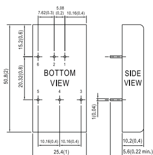
▲ RSDW20 2" x 1" x 0.4"
