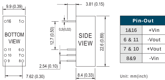
▲ SRS 0.89" x 0.39" x 0.33"
