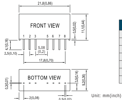
▲ SPAN02 0.86" x 0.36" x 0.44"
