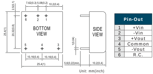
▲ DKMW20 1" x 1" x 0.40"
