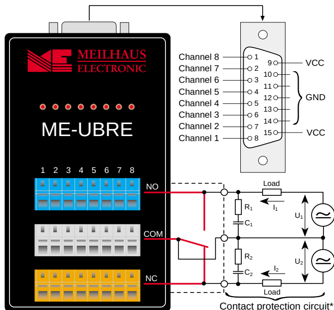
Diagram 1: Pinout
