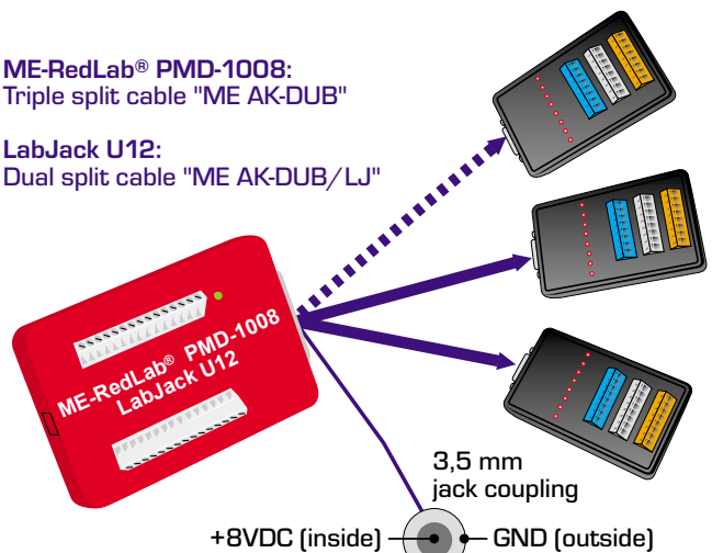
Diagram 2: Connection USB DAQ boxes
