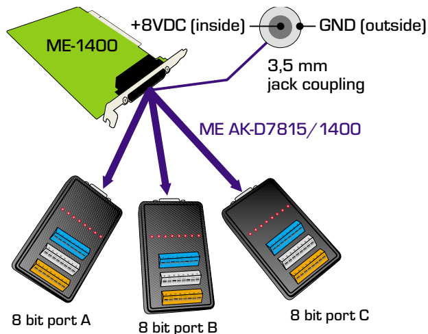
Diagram 3: Connection ME-1400/A/B
