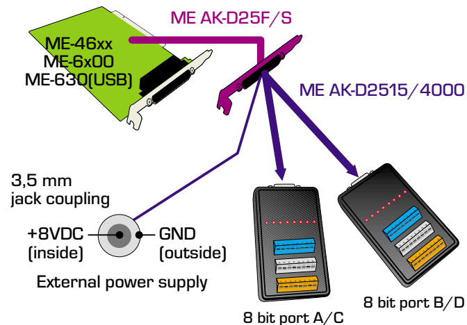
Diagram 4: Connection ME-Boards with ST2
