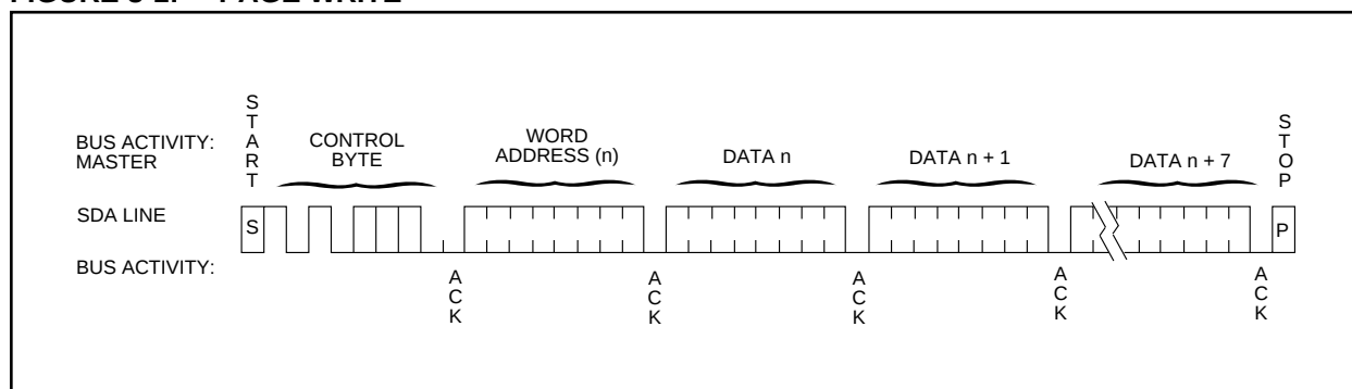
FIGURE 8-1: PAGE WRITE
