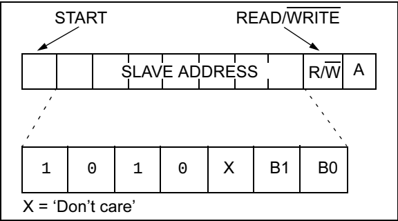
FIGURE 3-1: CONTROL BYTE ALLOCATION
