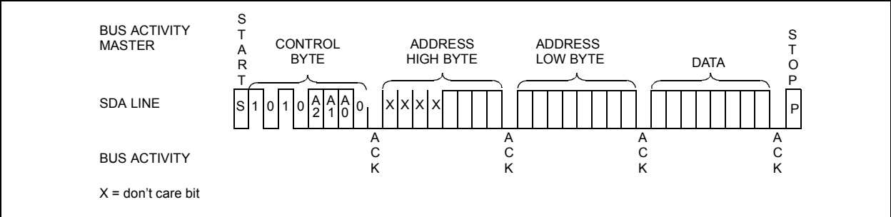
FIGURE 4-1: BYTE WRITE
