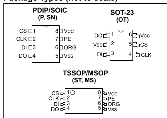
Package Types (not to scale)
