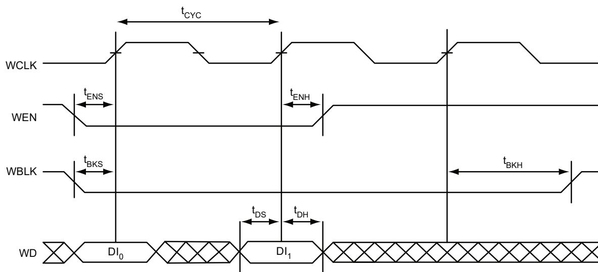
FIGURE 2-48: FIFO WRITE
