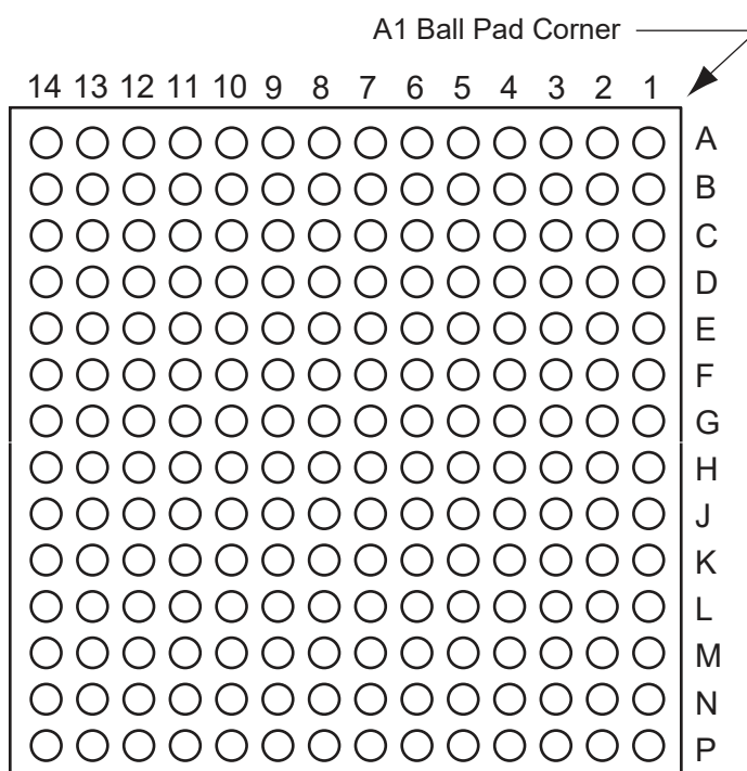
FIGURE 4-4: CS196—BOTTOM-VIEW
