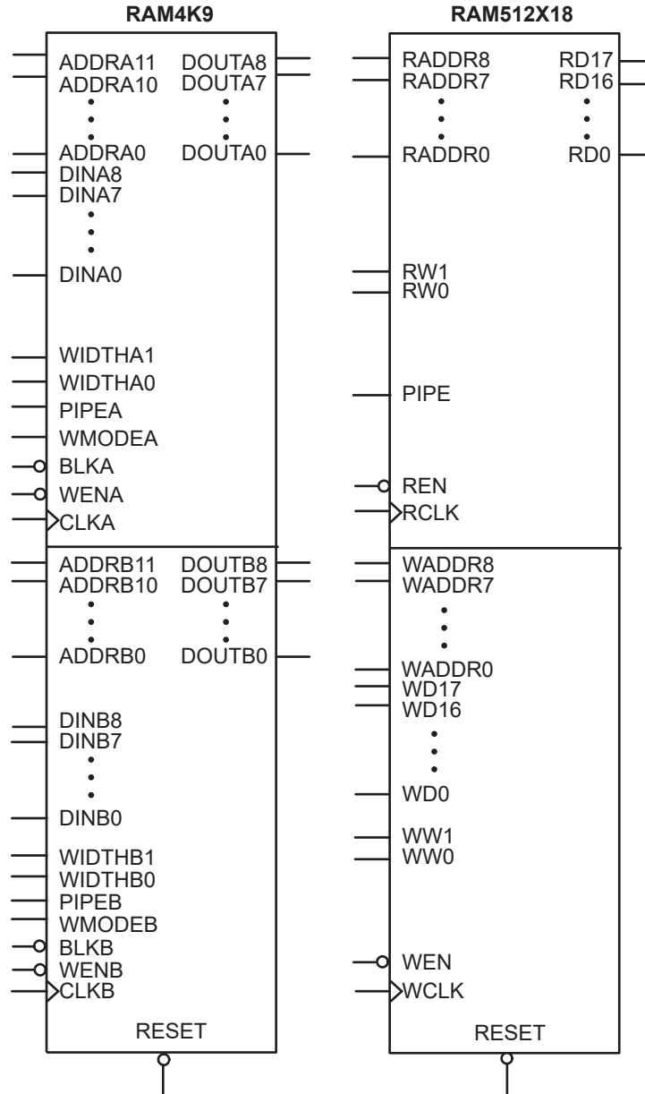
FIGURE 2-31: RAM MODELS
