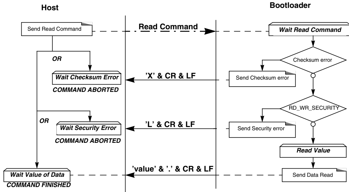
Figure 23-16. Read Flow
