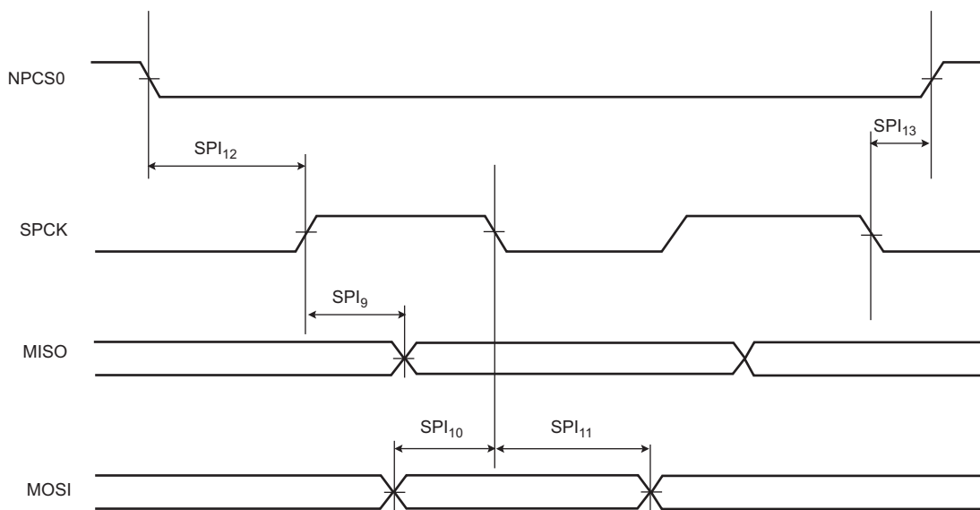
Figure 46-13. SPI Slave mode 1 and 2
