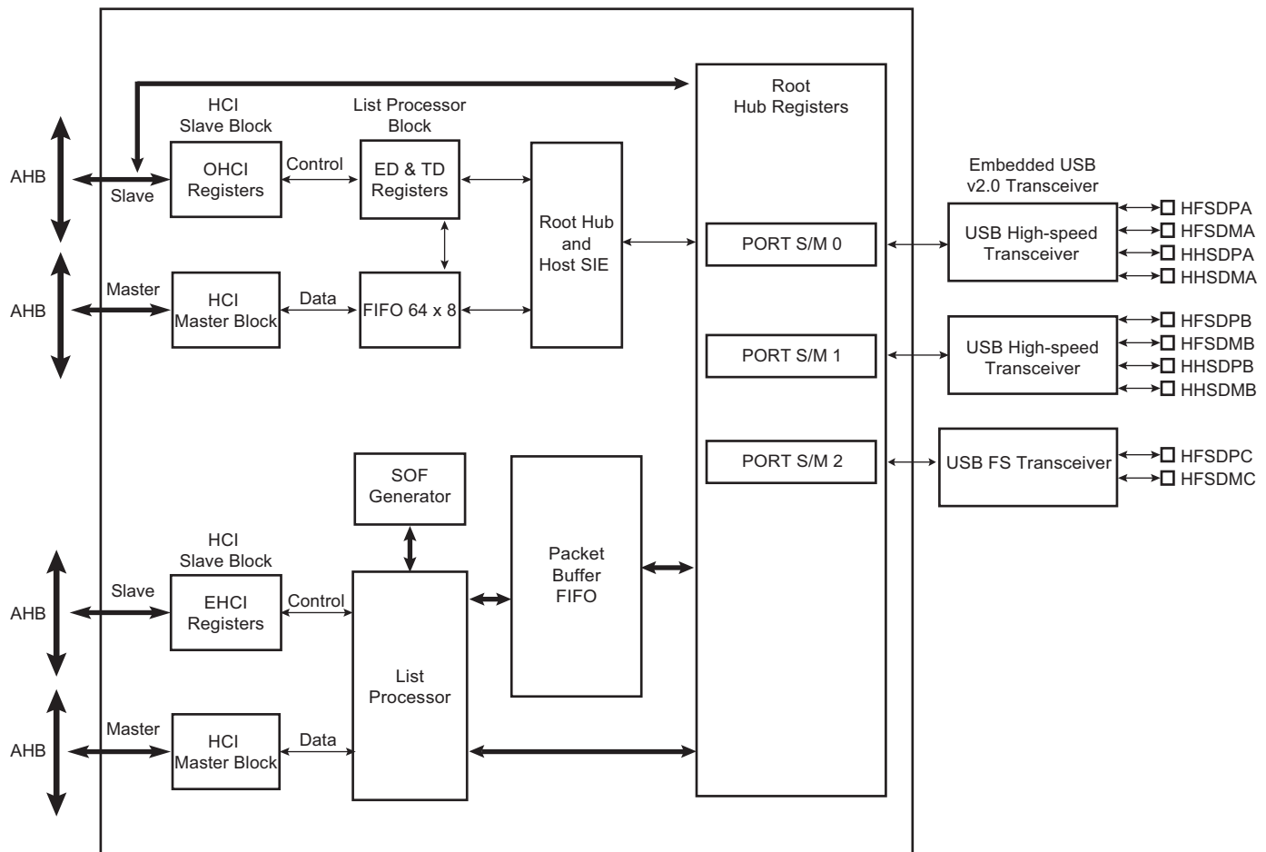
Figure 32-1. Block Diagram
