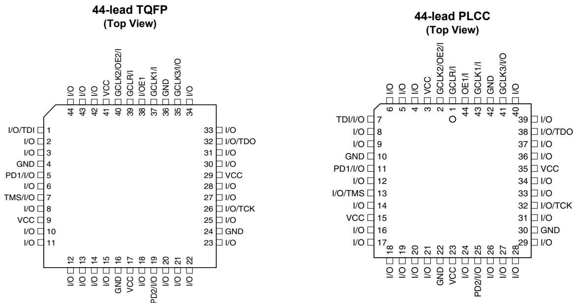
Figure 1-1. Pinouts
