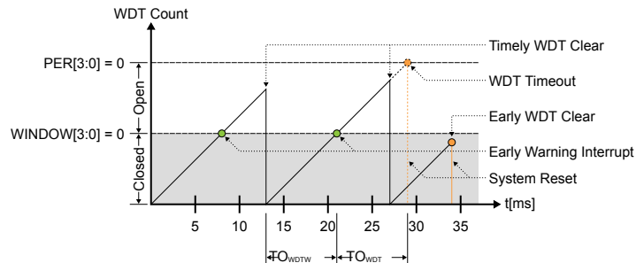
Figure 20-3. Window-Mode Operation
