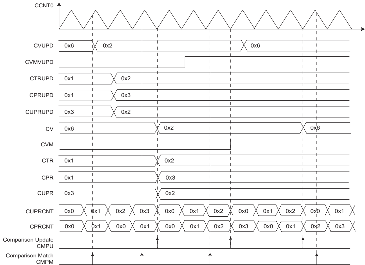
Figure 51-24. Comparison Waveform
