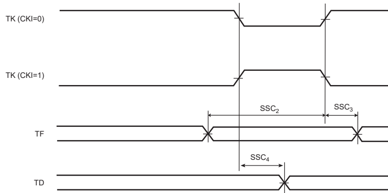
Figure 59-34. SSC Transmitter, TK and TF in Input
