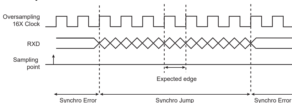
Figure 46-60. Bit Resynchronization
