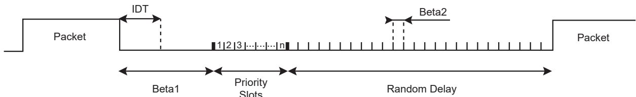
Figure 46-59. LON Timings
