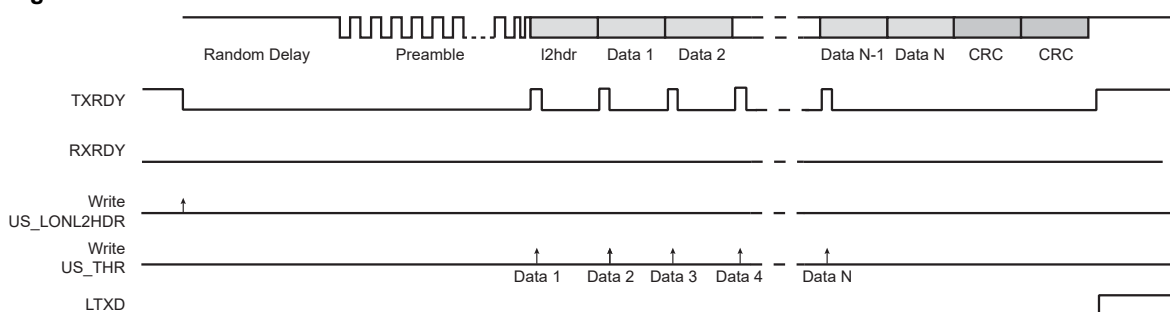
Figure 46-61. Tx Frame
