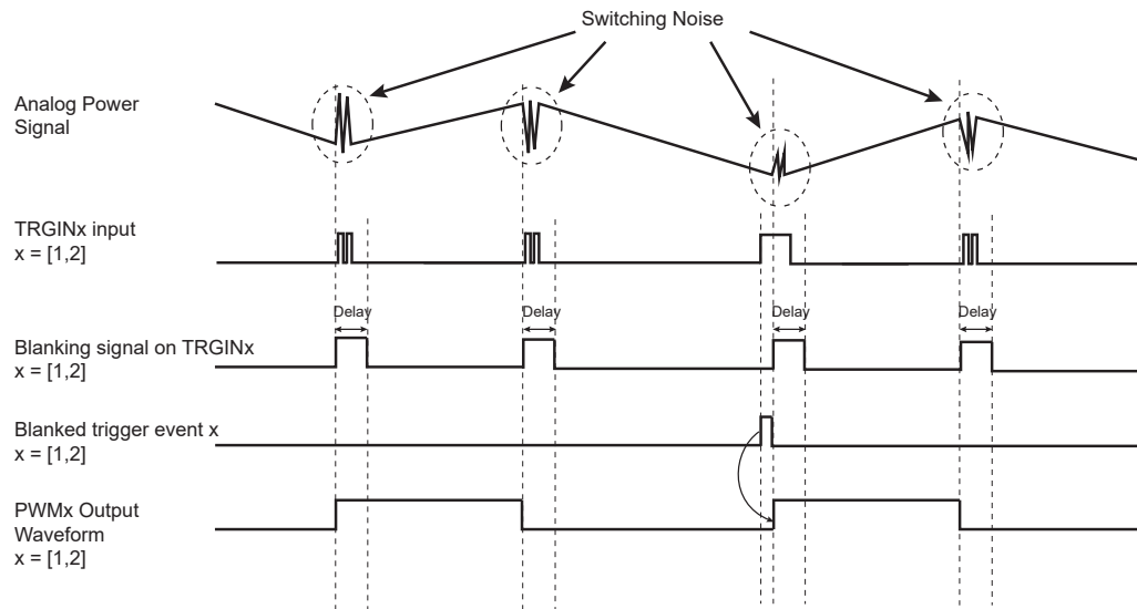
Figure 51-33. Leading-Edge Blanking
