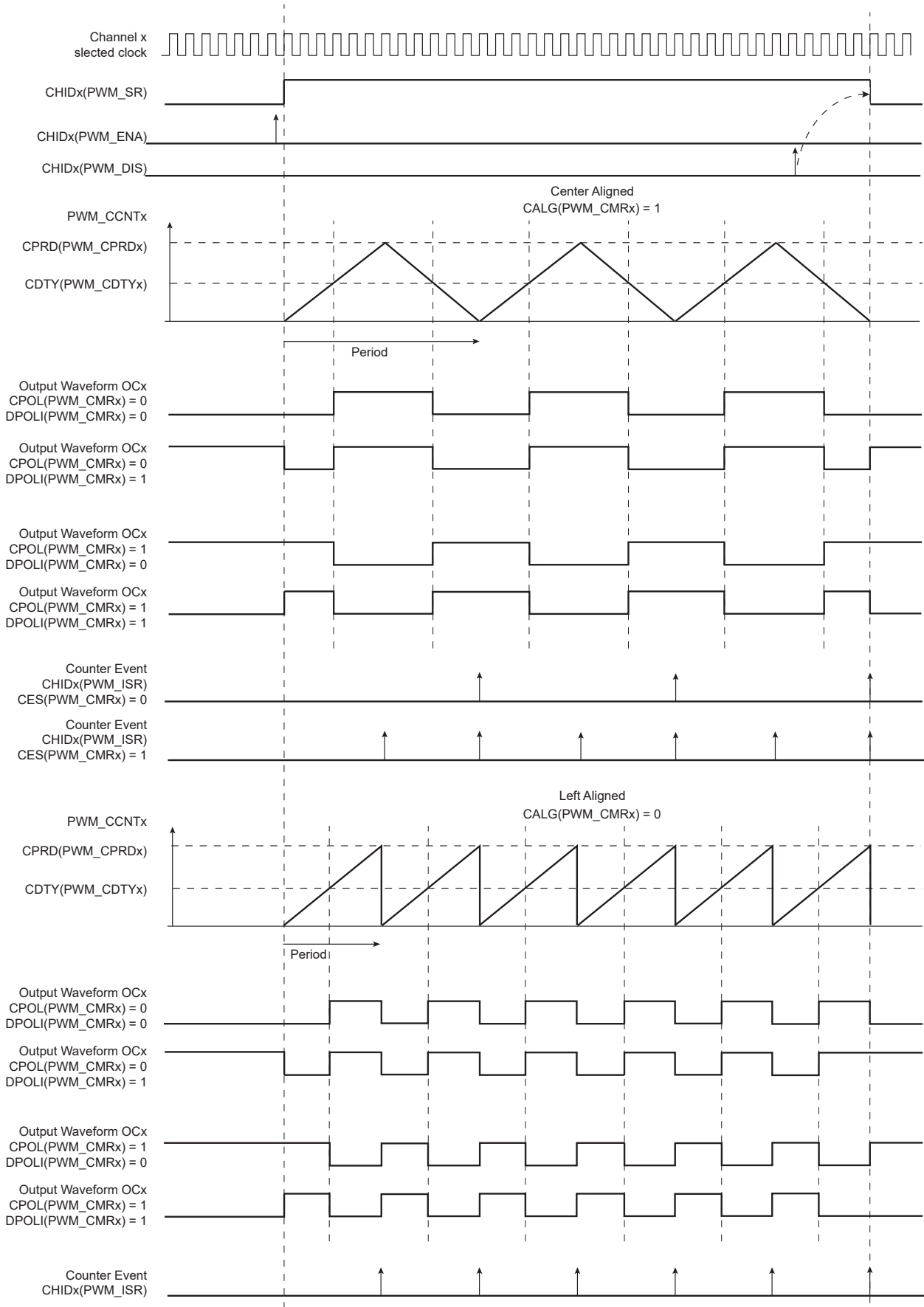
Figure 51-5. Waveform Properties
