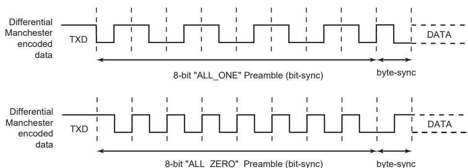
Figure 46-57. Preamble Patterns
