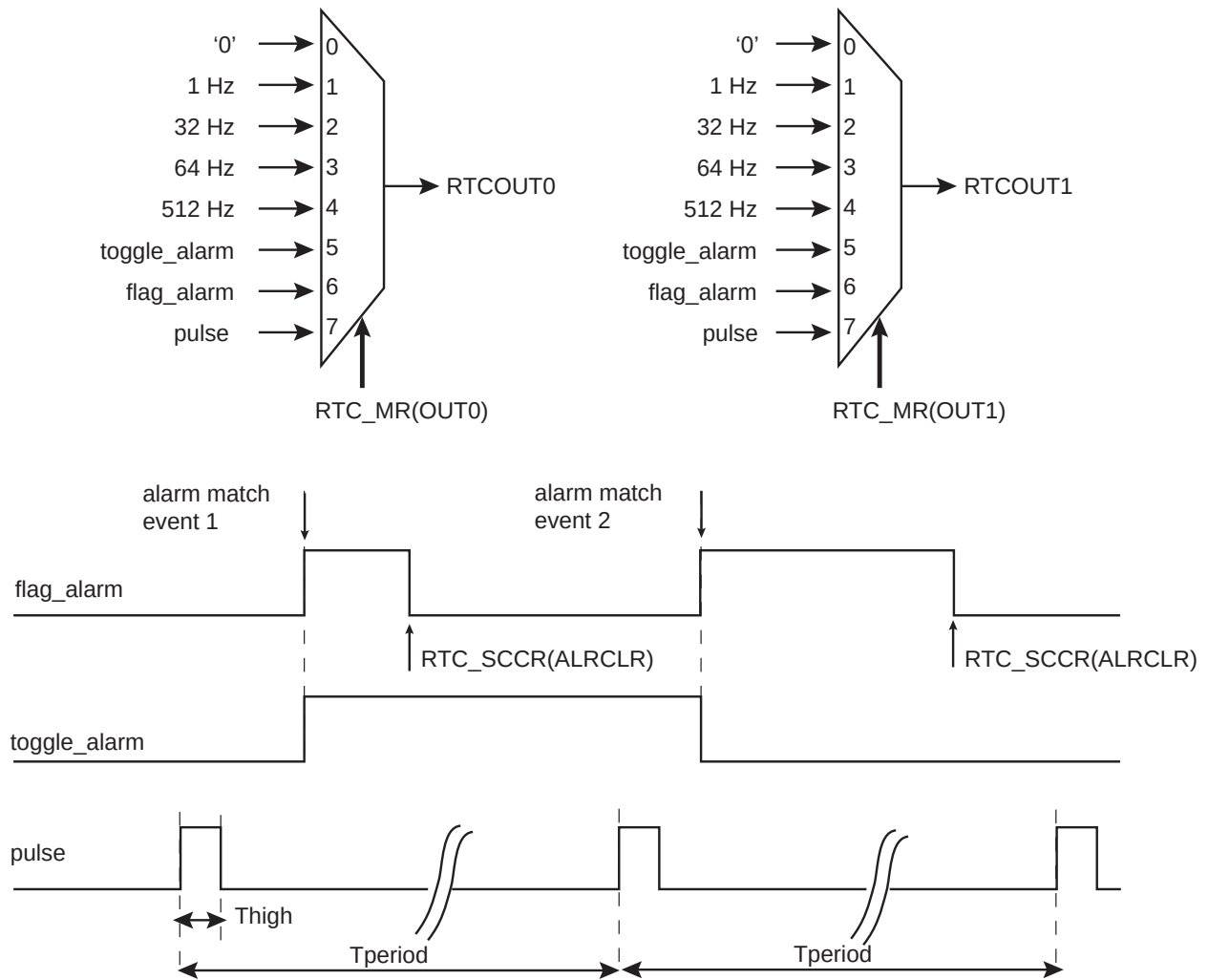
Figure 27-6. Waveform Generation
