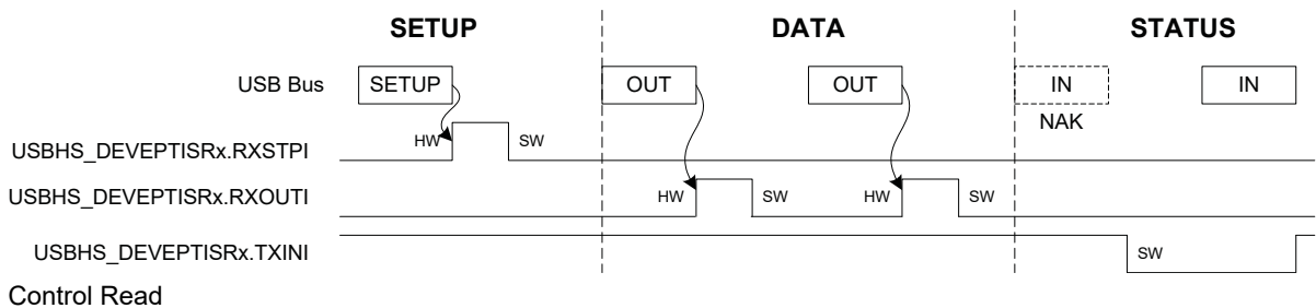
Figure 39-9. Control Write
