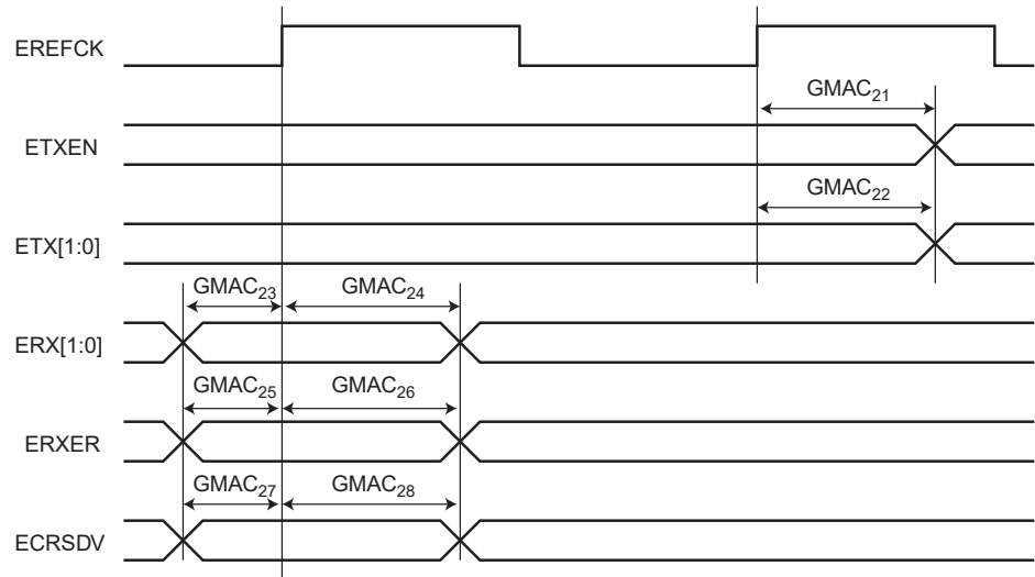
Figure 59-30. GMAC RMII Mode Signals
