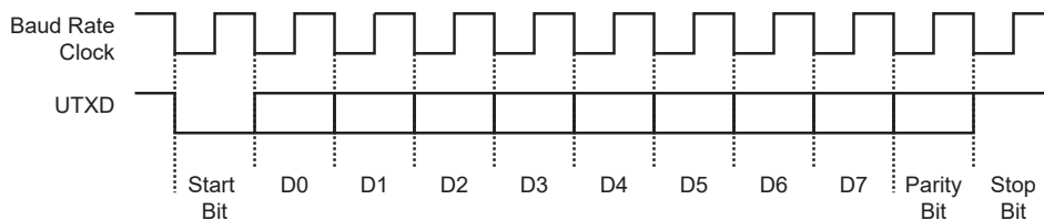
Figure 47-9. Character Transmission
