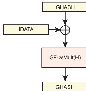
Figure 57-7. Single \text{GHASH}_H Block Diagram ( \text{AADLEN} \leq 0x10 and \text{CLEN} = 0 )
