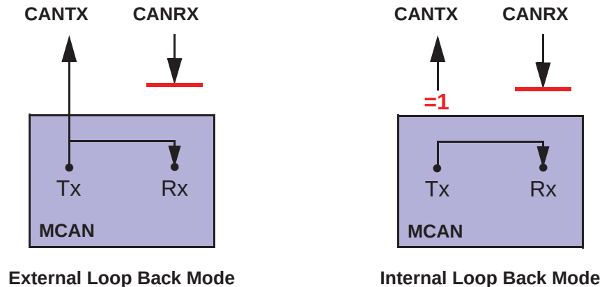
Figure 49-4. Pin Control in Loop Back Modes
