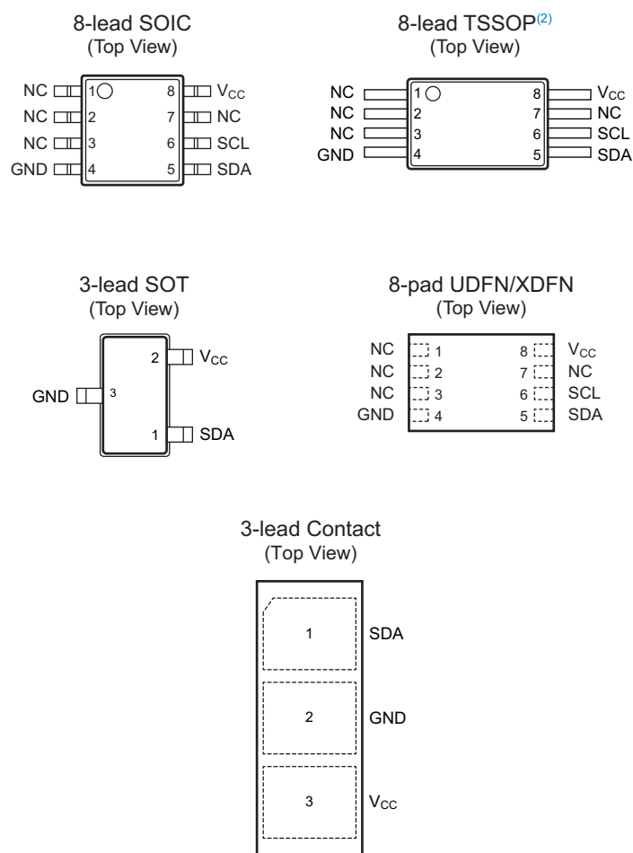
Figure 1. Pinouts (1)
