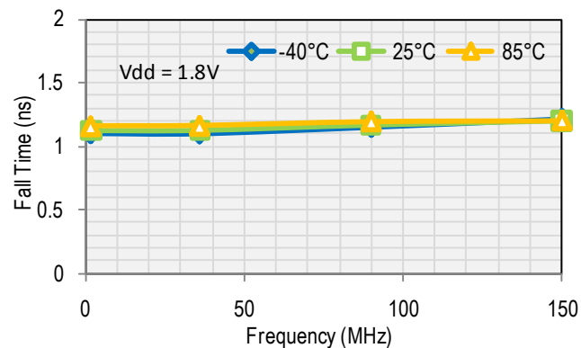
Fall Time
