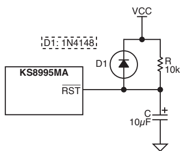
Figure 24. Recommended Circuit for Interfacing with CPU/FPGA Reset
