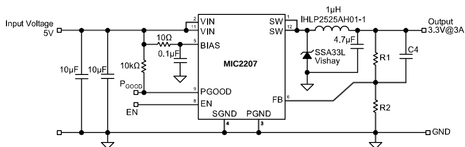
3A 2MHz Buck Regulator
