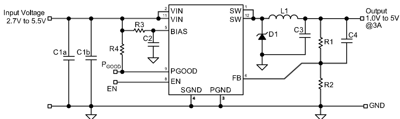
MIC2207 Schematic
