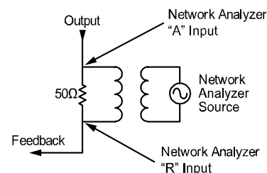
Figure 7. Transformer Injection
