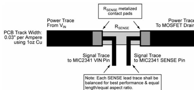
Figure 12. 4-Wire Kelvin Sense Connections for R_{\text{SENSE}}
