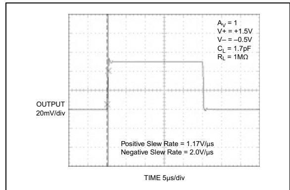
FIGURE 2-36: Large Signal Pulse Response.
