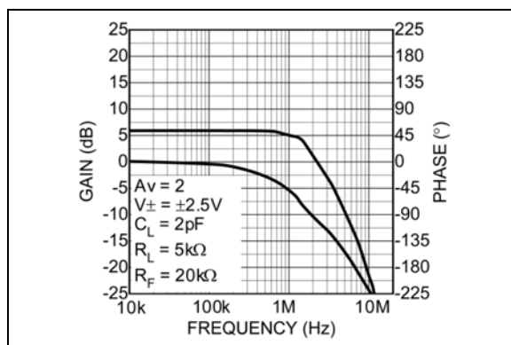
FIGURE 2-17: Gain Frequency Response.
