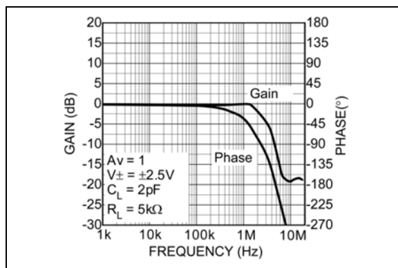
FIGURE 2-18: Unity Gain Frequency Response.
