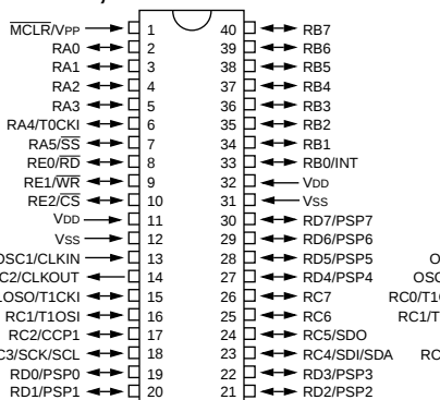
PIC16C64A PIC16CR64
