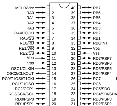
PIC16C64
