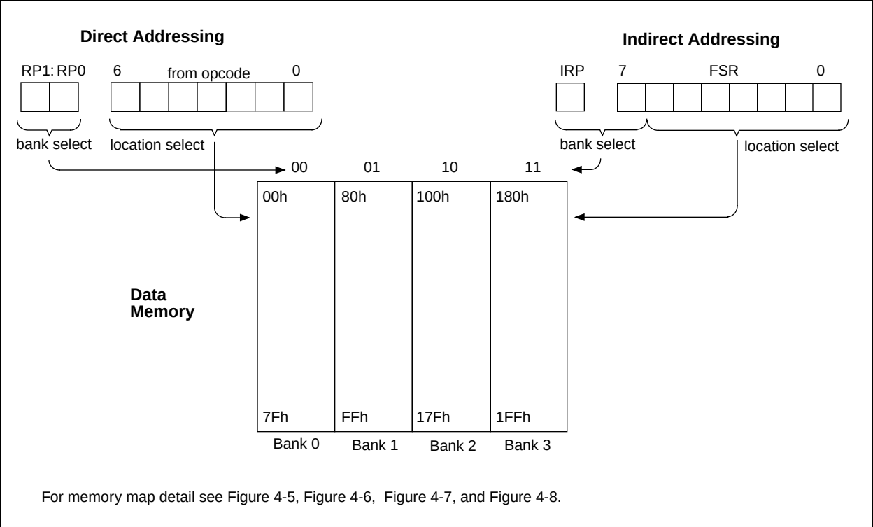
FIGURE 4-25: DIRECT/INDIRECT ADDRESSING
