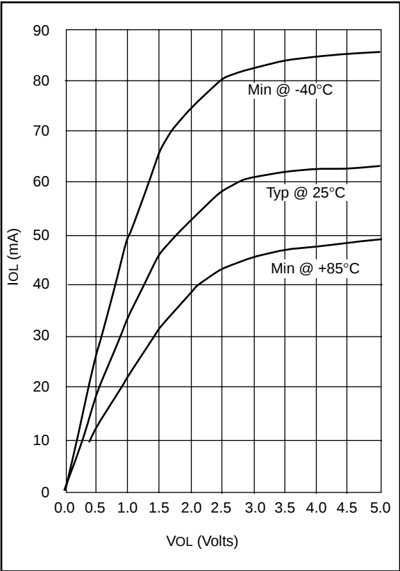
FIGURE 17-22: IOL vs. VOL, VDD = 5V
