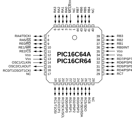
PLCC
