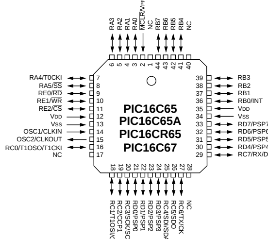
PLCC
