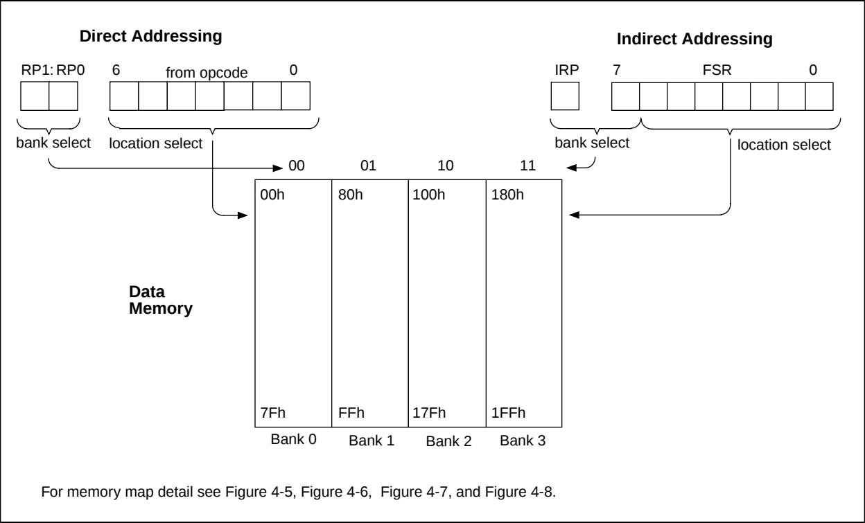
FIGURE 4-25: DIRECT/INDIRECT ADDRESSING
