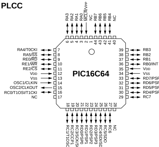
PLCC
