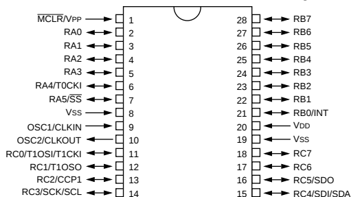
PIC16C62
