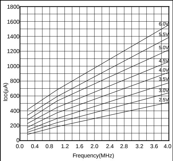
FIGURE 24-28: MAXIMUM I_{DD} vs. FREQUENCY (XT MODE, -40°C TO 85°C)
