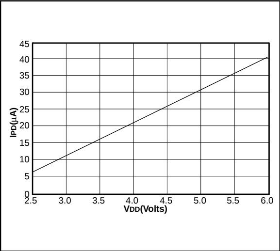
FIGURE 24-11: MAXIMUM I_{PD} vs. TIMER1 ENABLED (32 kHz, RC0/RC1 = 33 pF/33 pF, 85°C TO -40°C, RC MODE)
