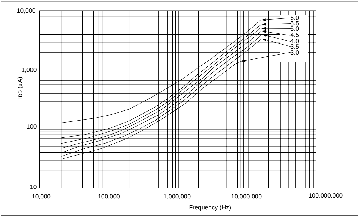
FIGURE 17-14: MAXIMUM I DD vs. FREQUENCY (EXTERNAL CLOCK, -55° TO +125°C)
