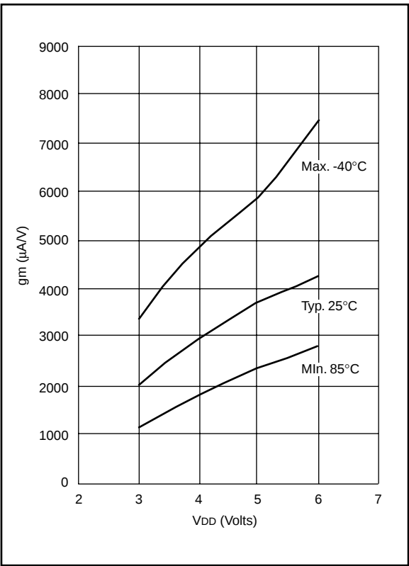
FIGURE 17-16: TRANSCONDUCTANCE (gm) OF HS OSCILLATOR vs. V DD
