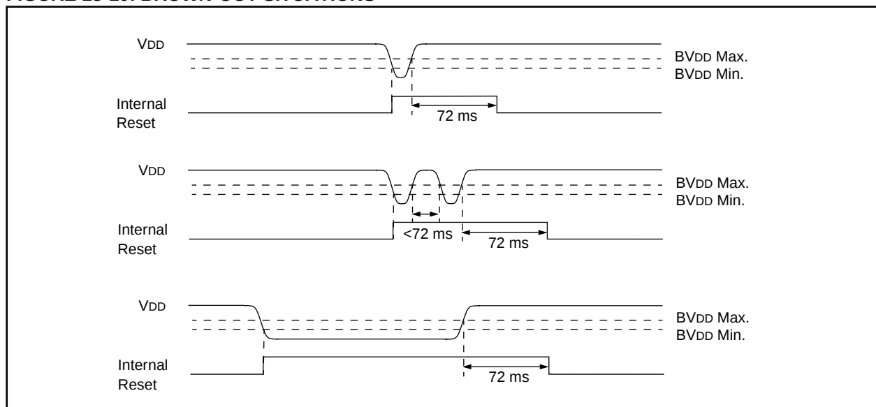
FIGURE 13-10: BROWN-OUT SITUATIONS
