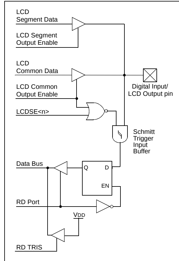
FIGURE 4-8: PORTF BLOCK DIAGRAM
