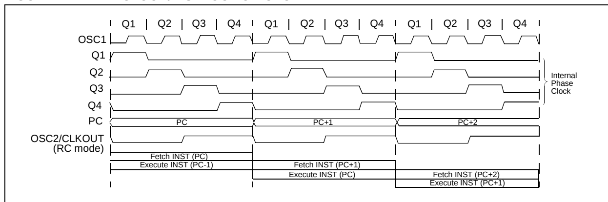
FIGURE 1-2: CLOCK/INSTRUCTION CYCLE
