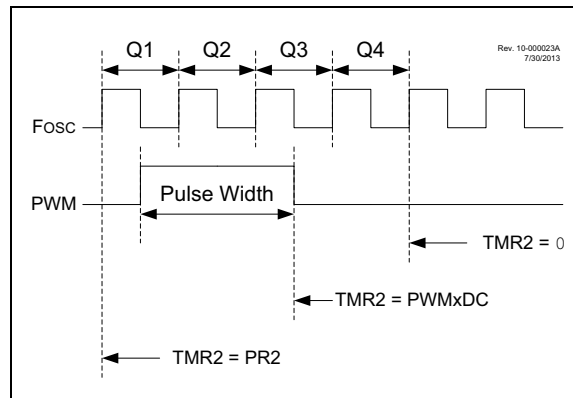
FIGURE 19-2: PWM OUTPUT
