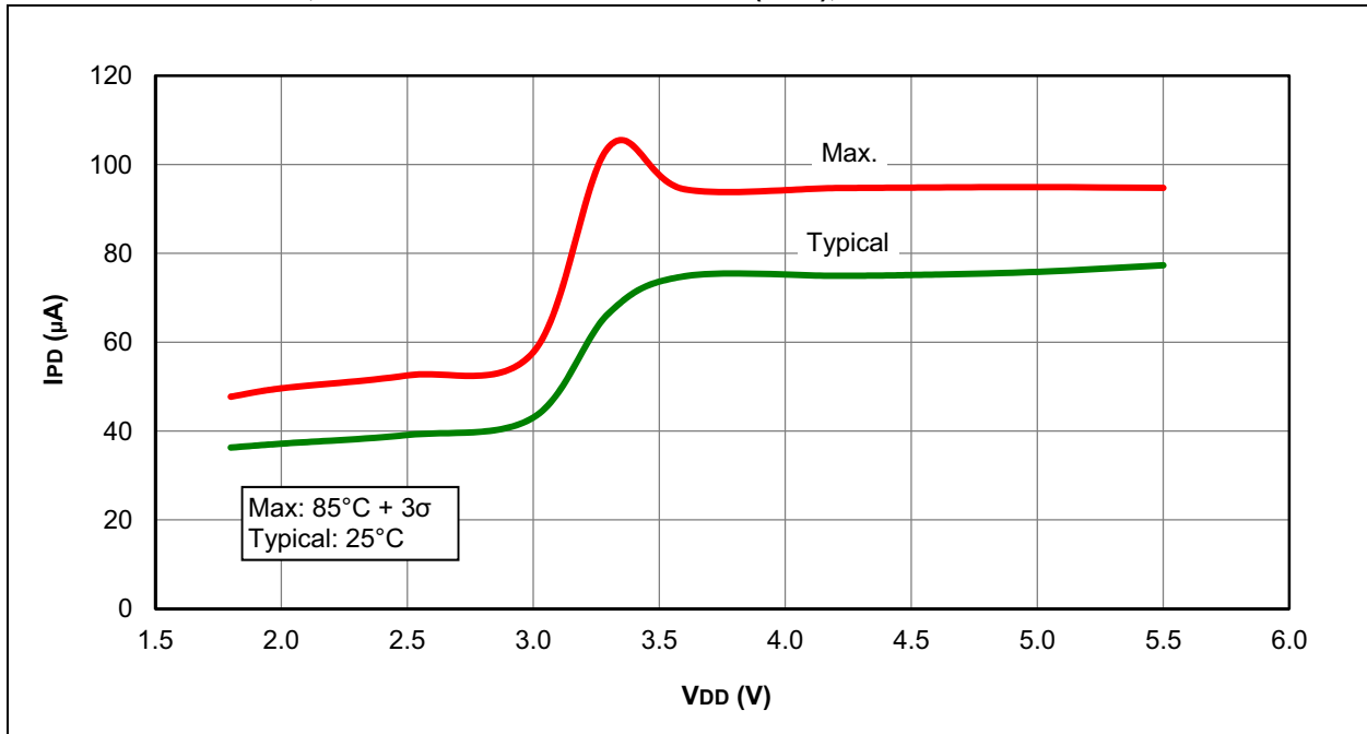
FIGURE 31-36: I_{PD} , FIXED VOLTAGE REFERENCE (FVR), PIC16F1938/9 ONLY
