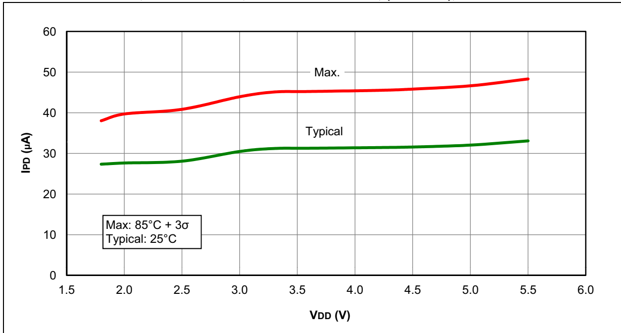
FIGURE 31-48: I_{PD} , COMPARATOR, LOW-POWER MODE, ( CxSP = 0 ), PIC16F1938/9 ONLY
