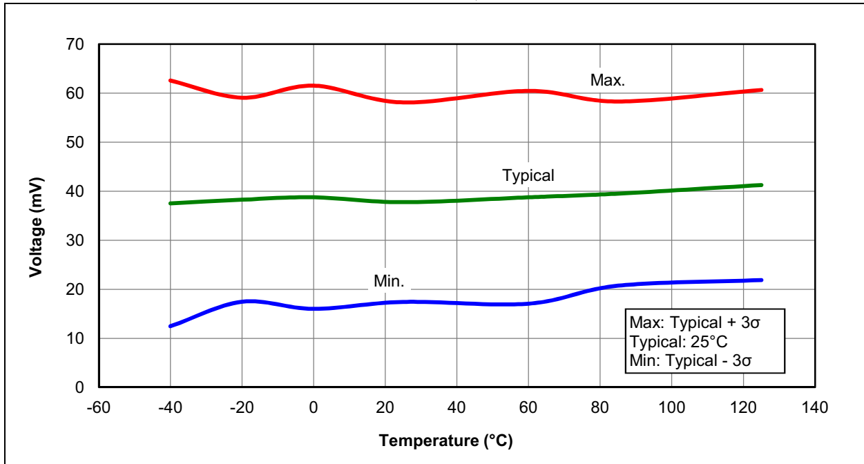
FIGURE 31-60: BROWN-OUT RESET HYSTERESIS, BORV = 1
