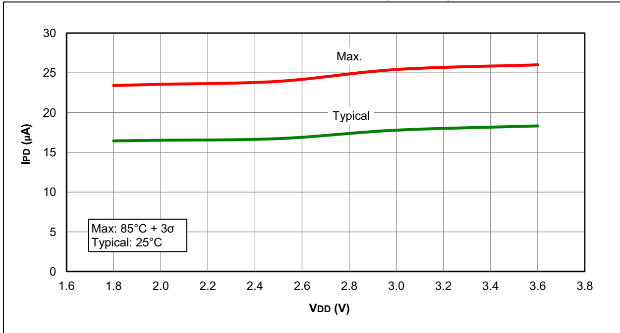
FIGURE 31-47: I_{PD} , COMPARATOR, LOW-POWER MODE, ( CxSP = 0 ), PIC16LF1938/9 ONLY
