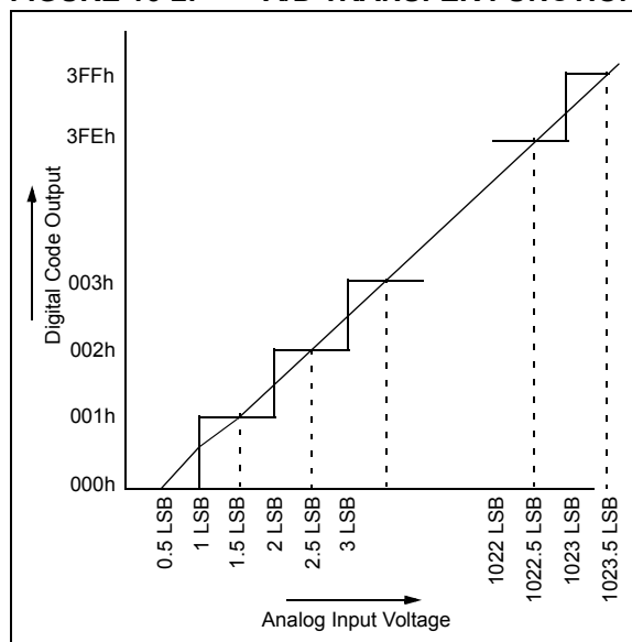
FIGURE 16-2: A/D TRANSFER FUNCTION
