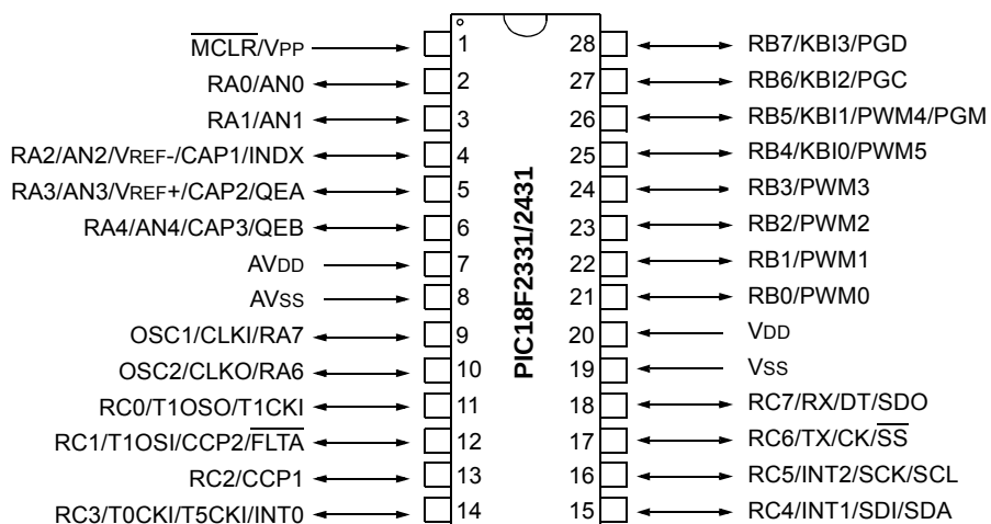
28-Pin SPDIP, SOIC
