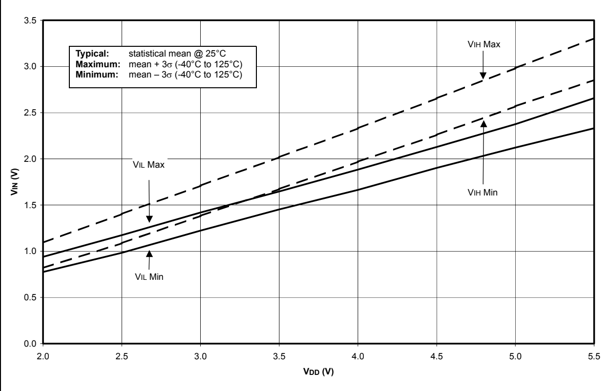
FIGURE 28-27: MINIMUM AND MAXIMUM V_{IH} vs. V_{DD} ( I^2C INPUT, -40^{\circ}C TO +125^{\circ}C )
