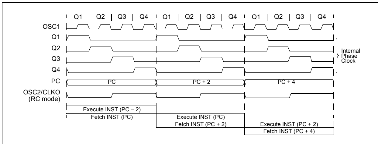
FIGURE 6-5: CLOCK/INSTRUCTION CYCLE
